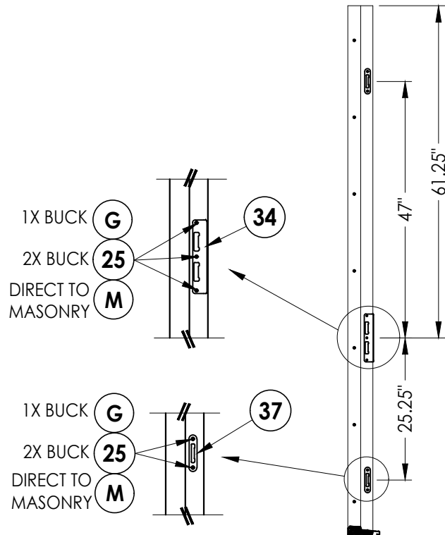
MULTI-POINT LOCK STRIKE PLATE DETAILS
